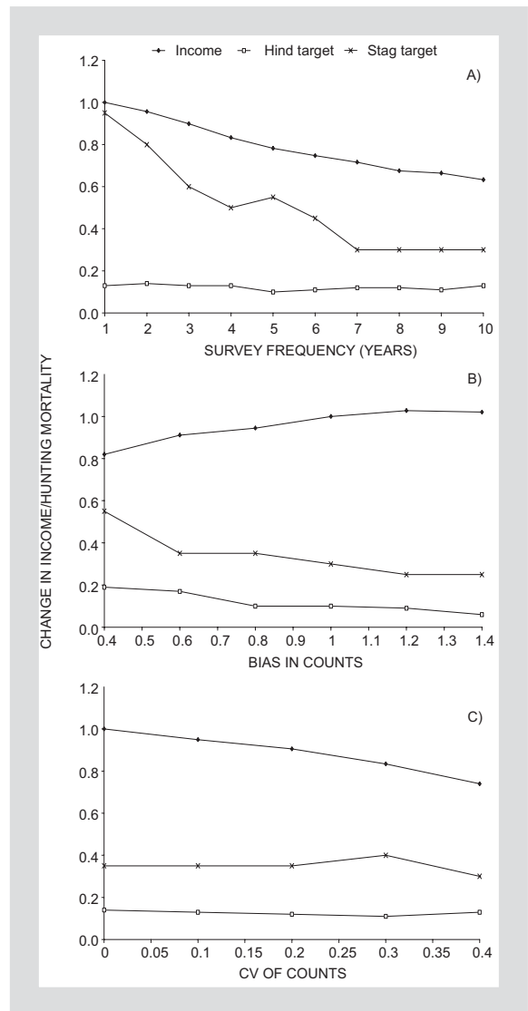
Figure 7. Effect of changes in data quality on income and hunting mortalities. Income is shown as the maximum obtainable (at the optimal hunting mortality) for a given data quality, normalised to that obtained under a perfect survey ('Change'). Target hunting mortalities are shown for both hinds and stags. In each case, one parameter is changed while the others are held constant at the values for a poor survey (see Table 3). The ranges tested encompass likely variation in data quality for Scottish estates. In A) the survey frequency varies between annual and once every 10 years; in B) the bias in the counts varies from 0.4 (on average the count is 40% lower than the actual population size) to 1.4 (40% higher than the actual population size) and in C) the coefficient of variation (CV) of the counts varies from 0 (no variability) to 0.4 (standard deviation is 40% of the mean).
